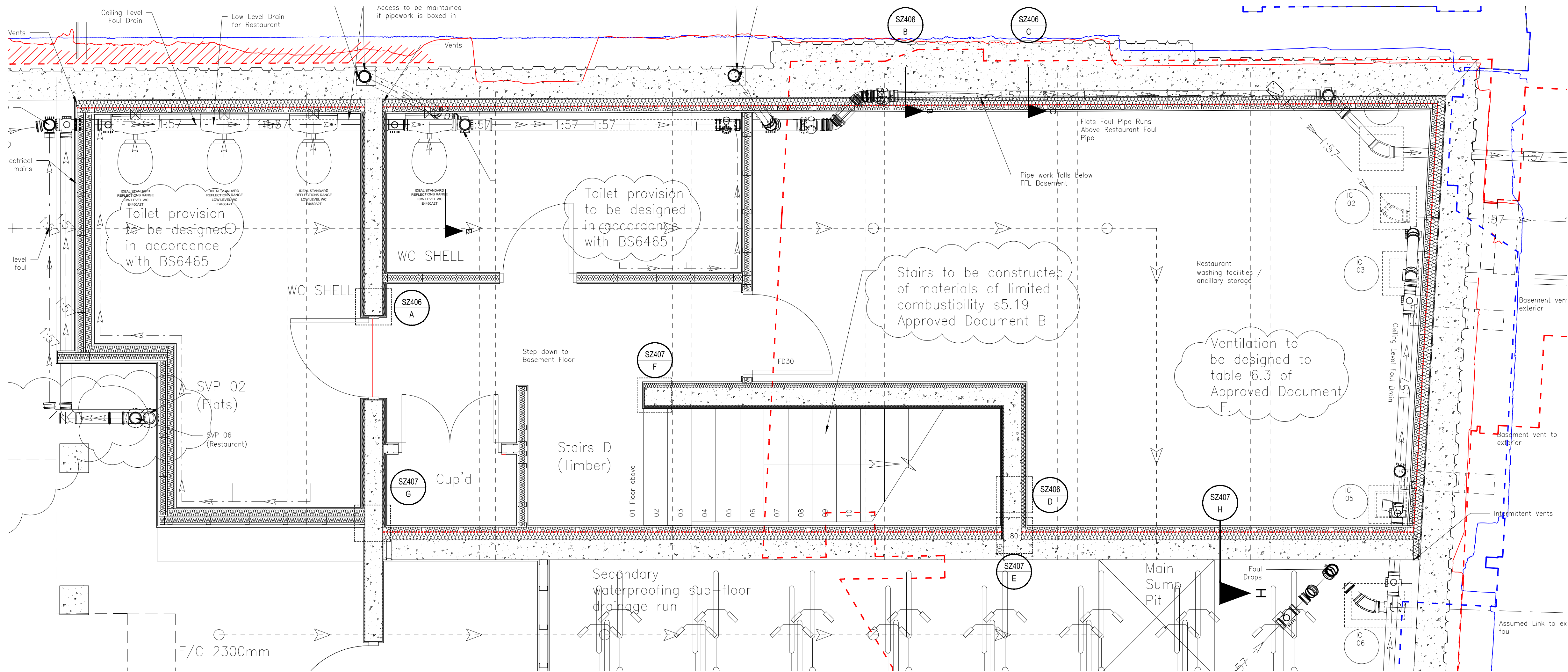
- Basement Plan Scale 1:25
